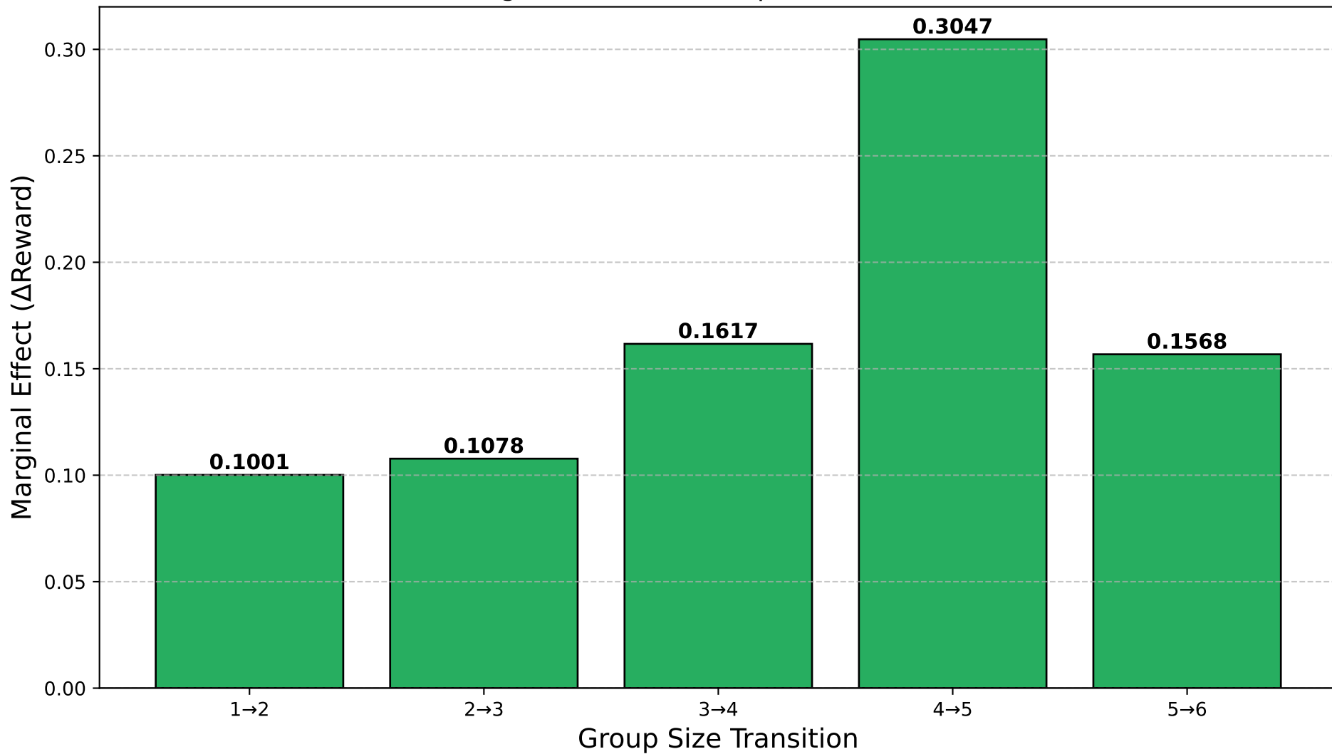
Marginal Effect of Group Size on Reward
